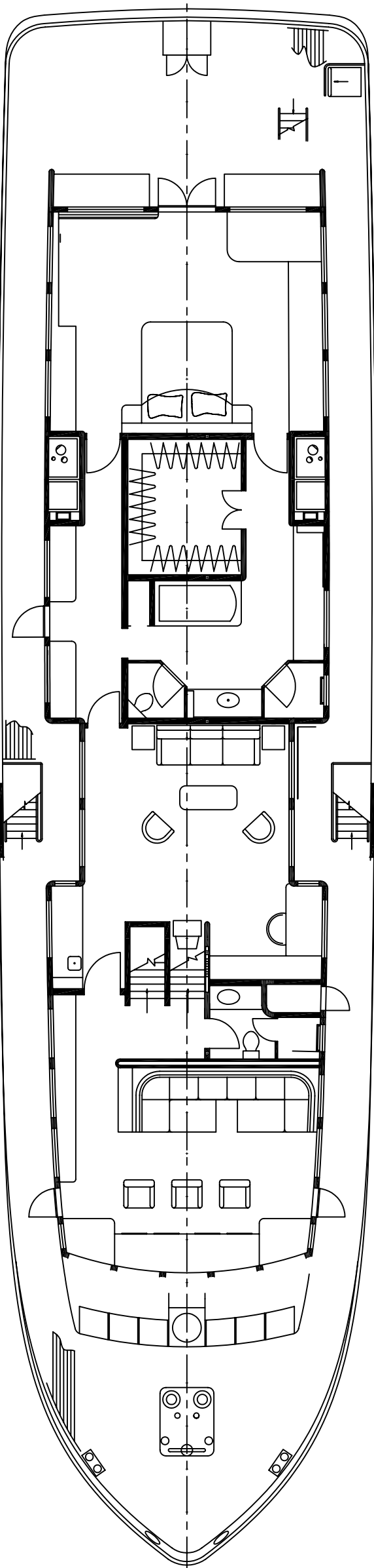
UPPER DECK
